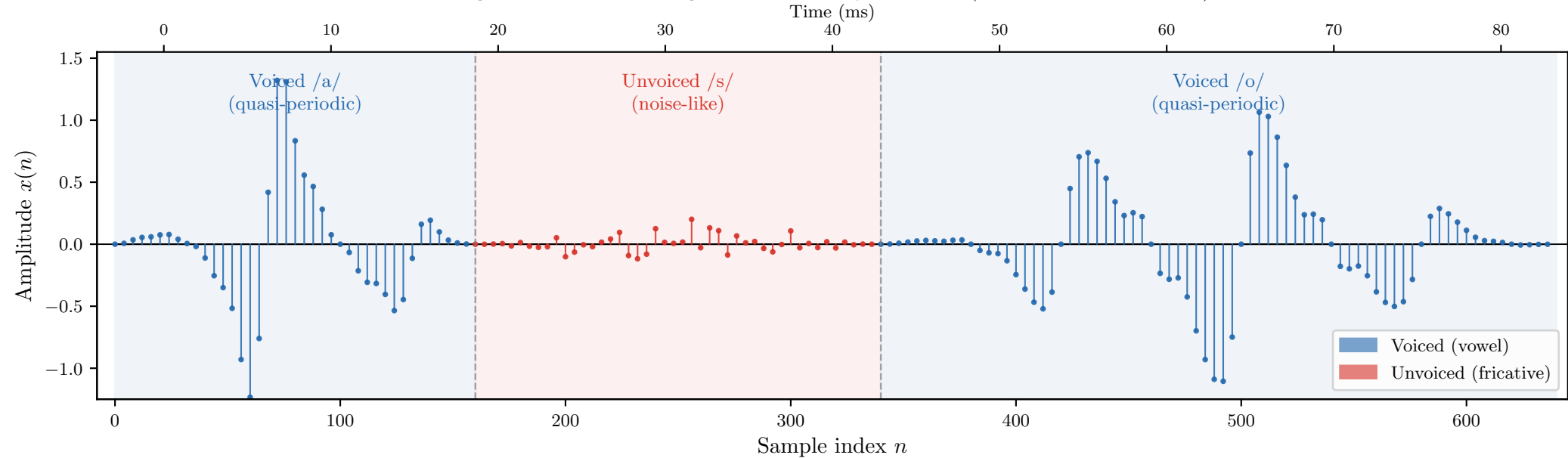
Figure 1.1 — Speech signal sampled at f_s = 8 kHz (discrete-time sequence)
